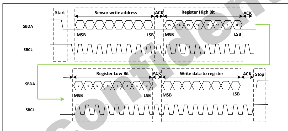
Figure 5-1 Writing Operation (2 bytes address – 1 byte data)
