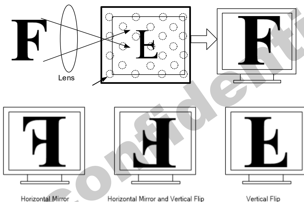
Figure 4-1 Readout Direction
