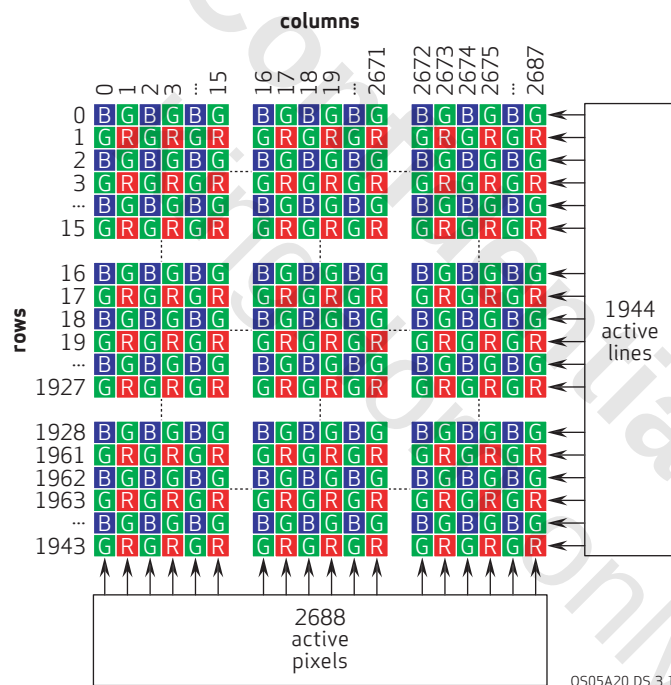
figure 3-1 sensor output pattern (2688x1944)
