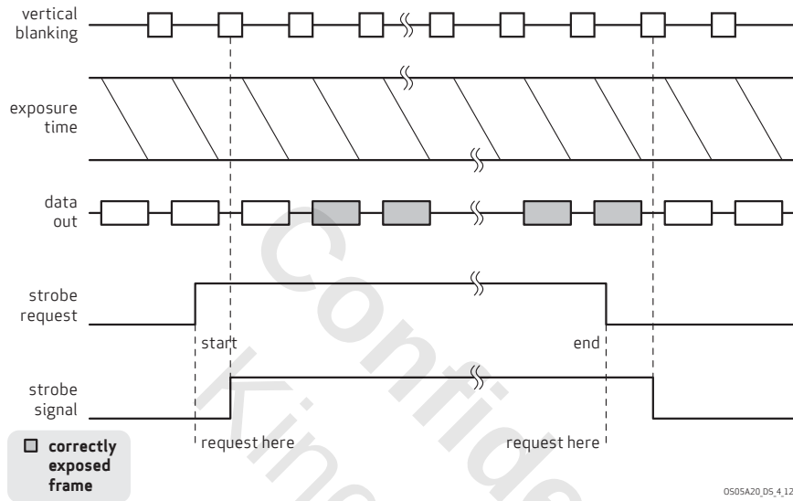
figure 4-12 LED 3 mode
