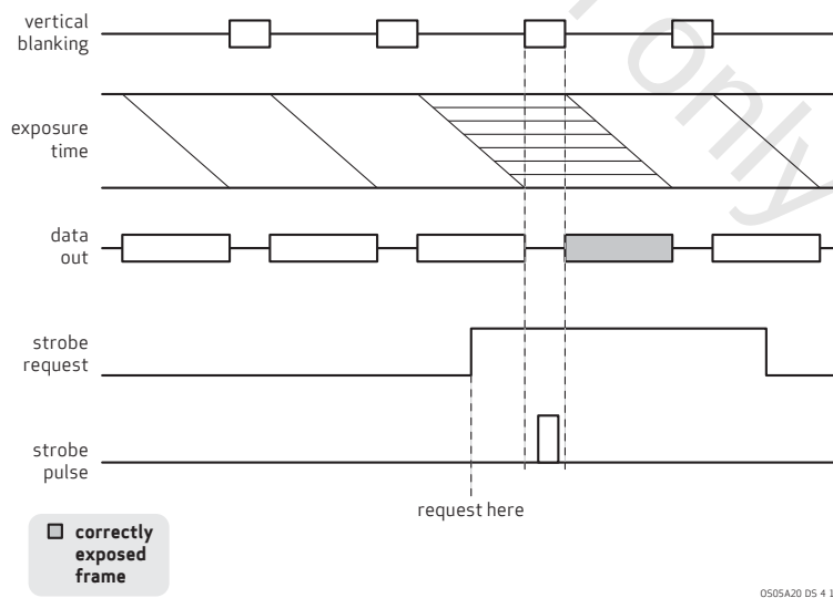
figure 4-13 LED 4 mode
