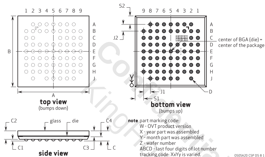
figure 8-1 package specifications
