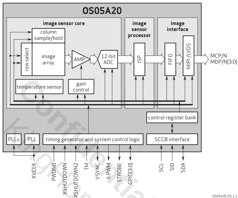
figure 2-1 OS05A20 block diagram
