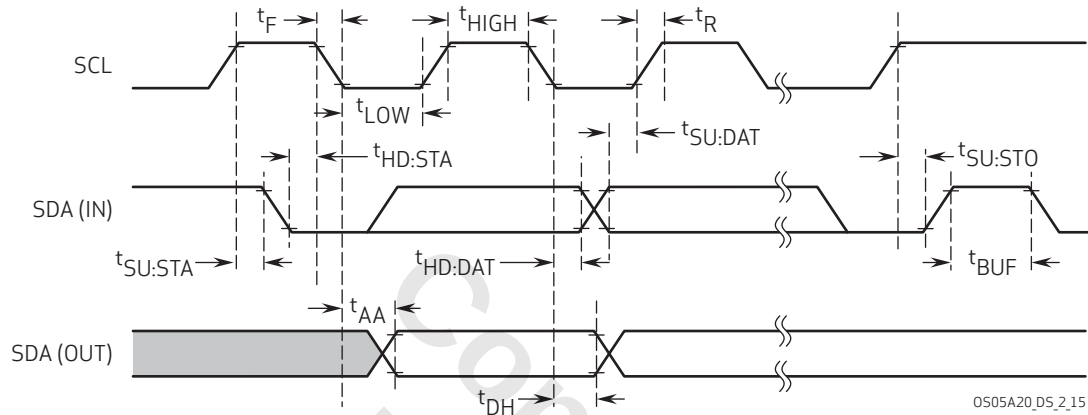
figure 2-15 SCCB interface timing
