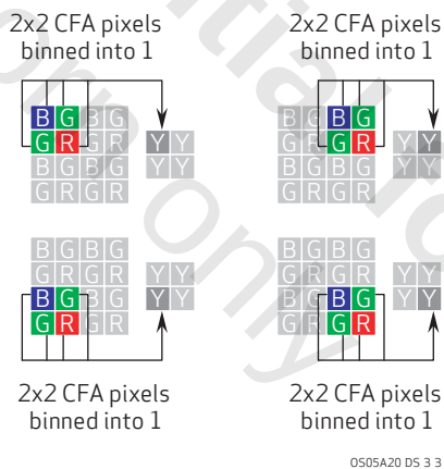
figure 3-3 example of 2x2 mono binning
