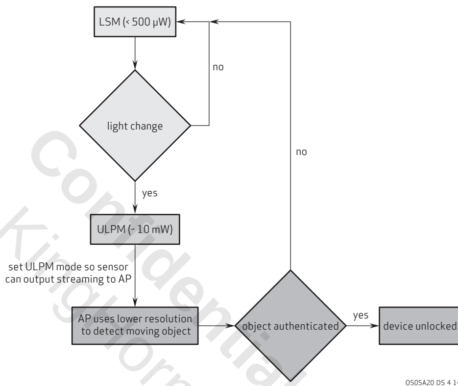
figure 4-15 LSM interrupt mode 1 configuration
