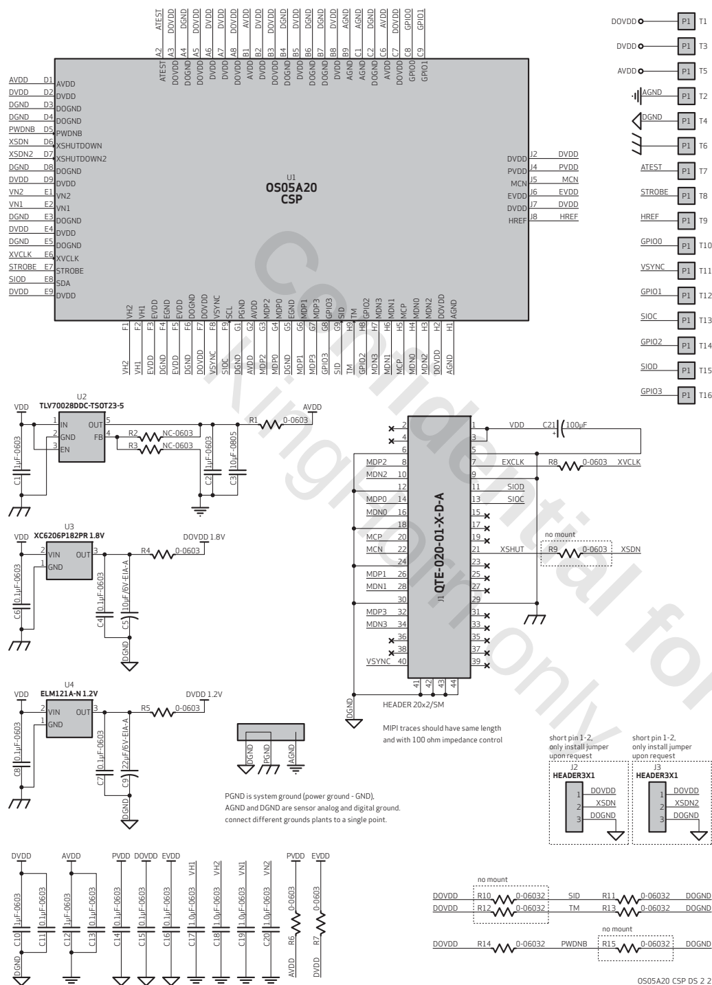
figure 2-2 OS05A20 reference schematic
