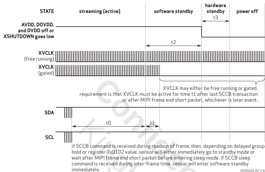
figure 2-6 power down sequence
