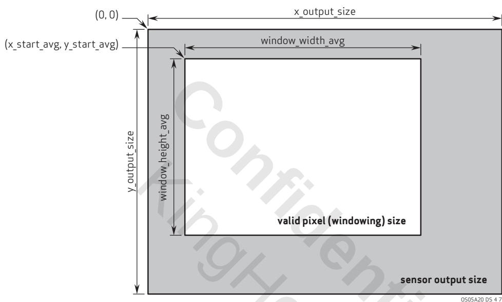
figure 4-7 average based window definition
