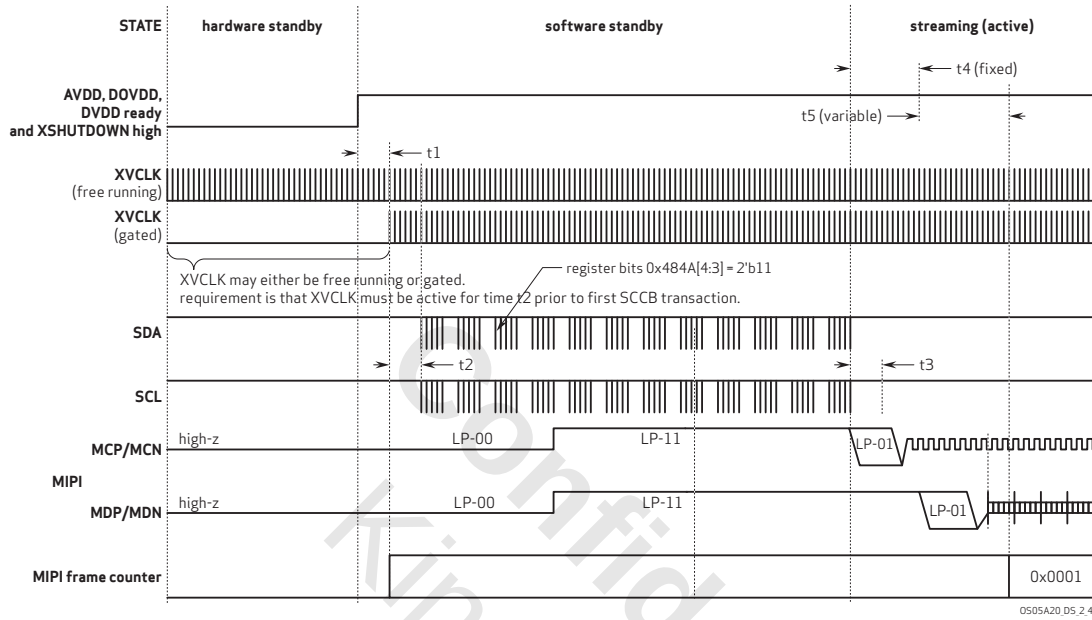
figure 2-4 power up sequence
