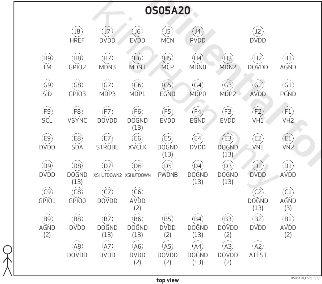
figure 1-1 pin diagram
