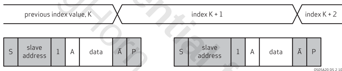
figure 2-10 SCCB single read from current location
