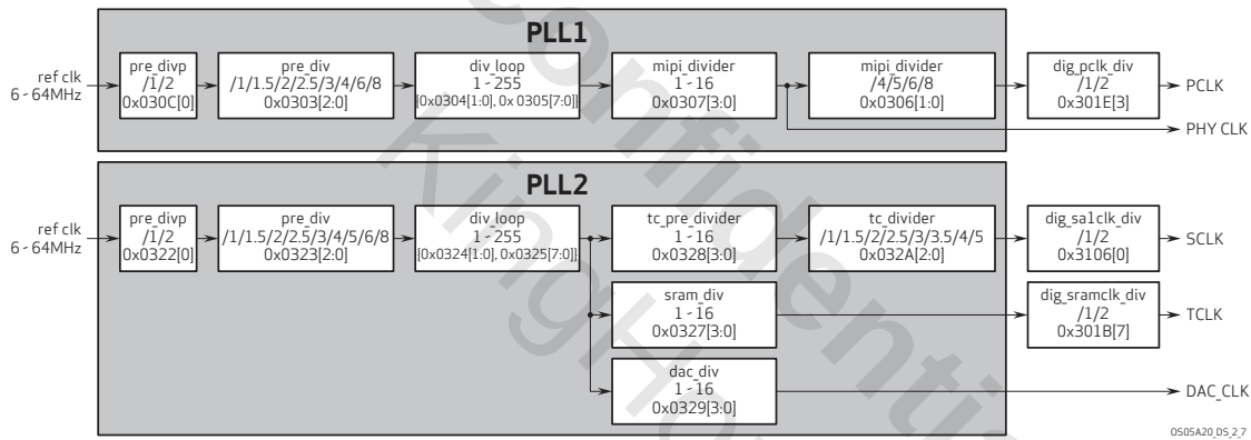
figure 2-7 clock scheme
