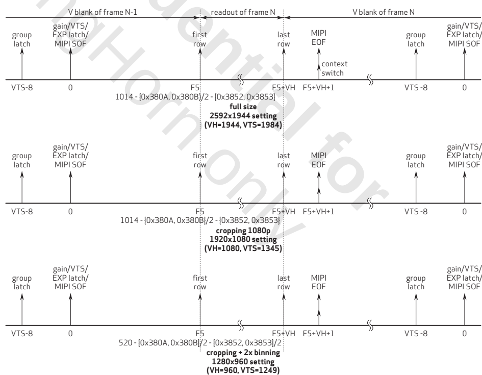
figure 2-3 exposure/gain latch points
