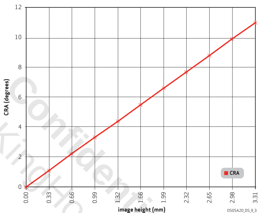
figure 9-3 chief ray angle (CRA)
