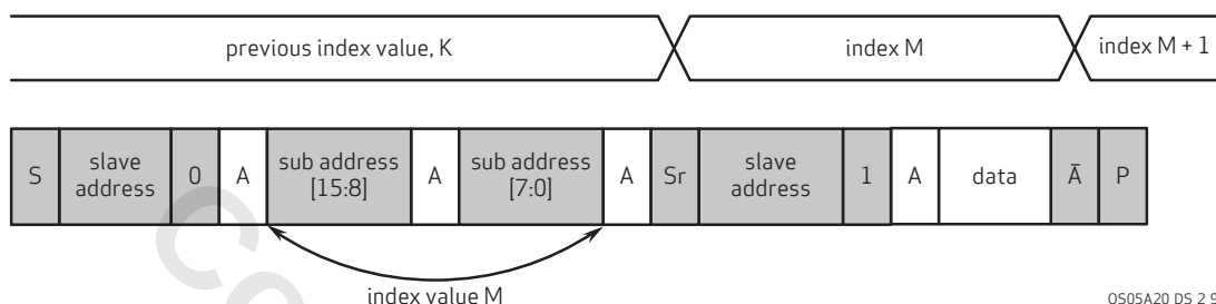
figure 2-9 SCCB single read from random location
