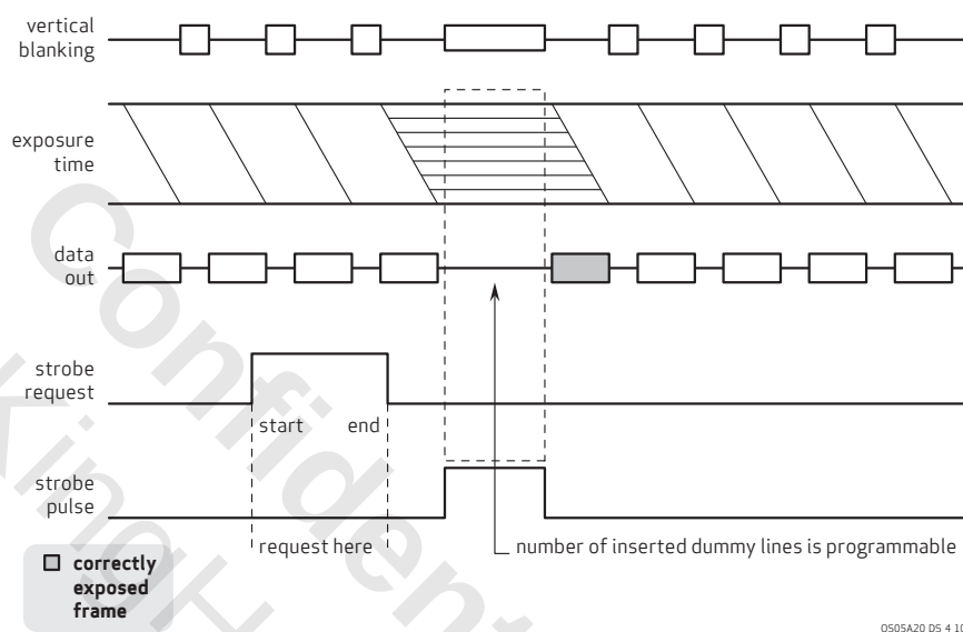
figure 4-11 LED 1 & 2 mode (part b)
