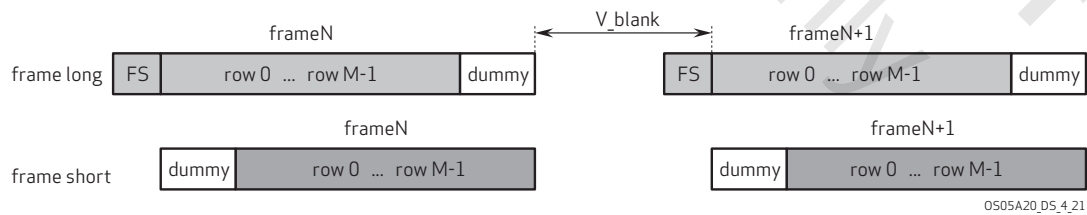
figure 4-21 set staggered HDR with no VC
