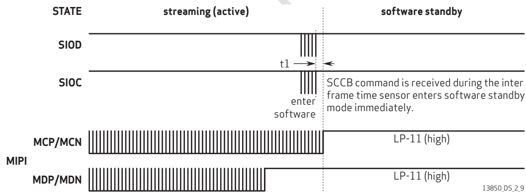
figure 2-9 standby timing (case 2)
