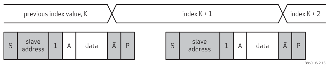
figure 2-13 SCCB single read from current location
