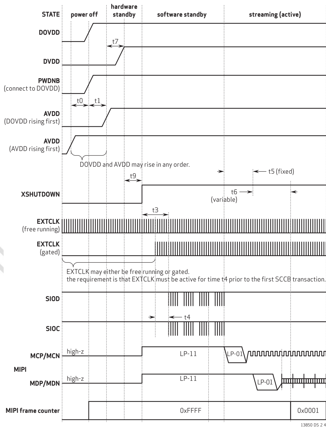
figure 2-4 power up sequence (case 1)
