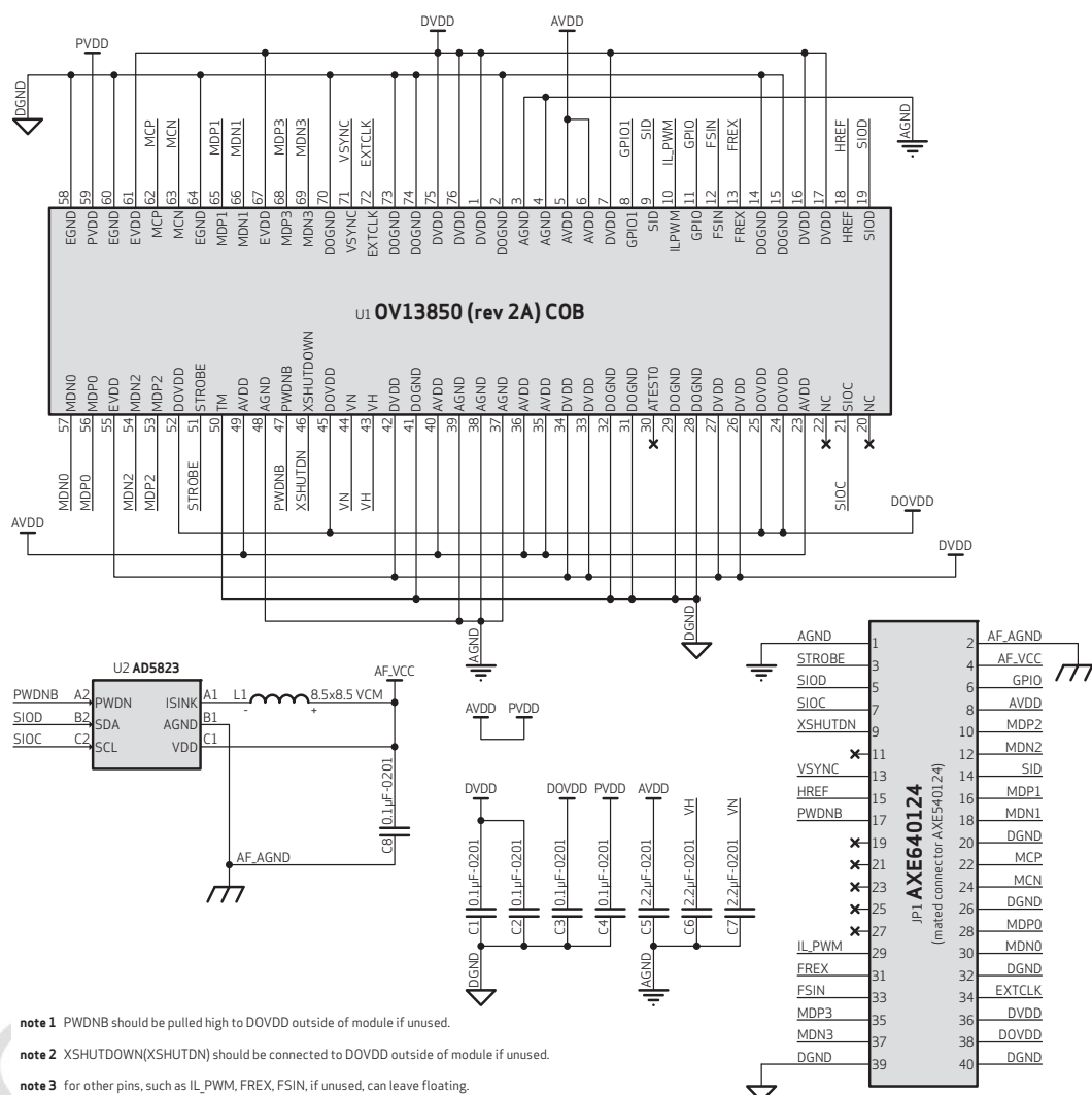
figure 2-2 OV13850 reference design schematic
