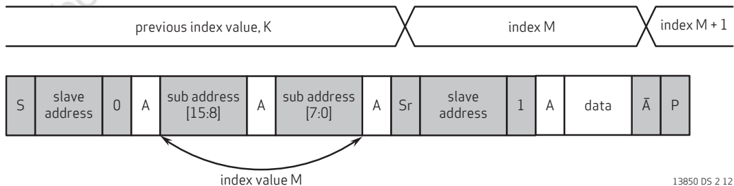
figure 2-12 SCCB single read from random location
