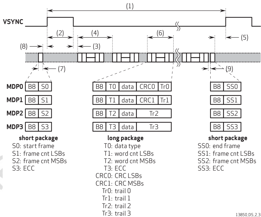
figure 2-3 MIPI timing
