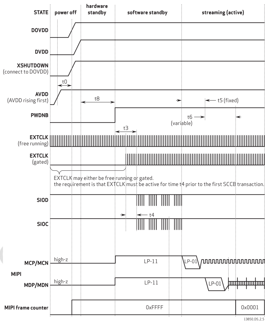
figure 2-5 power up sequence (case 2)
