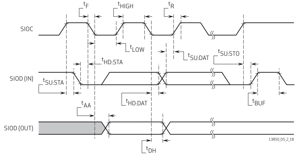
figure 2-18 SCCB interface timing
