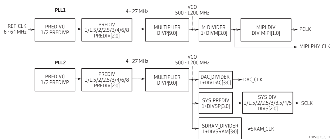
figure 2-10 OV13850 PLL diagram
