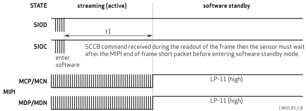
figure 2-8 standby timing (case 1)
