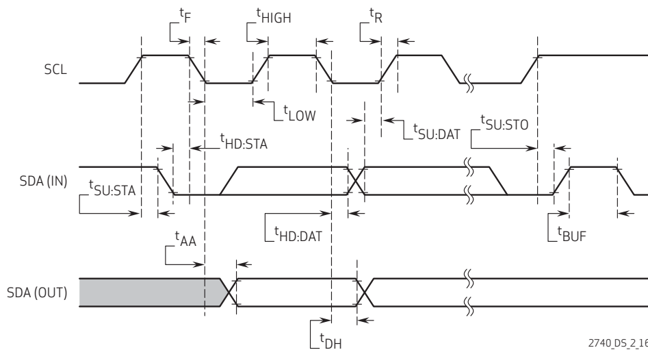
figure 2-16 SCCB interface timing
