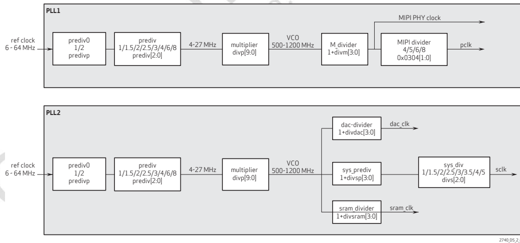
figure 2-8 clock scheme
