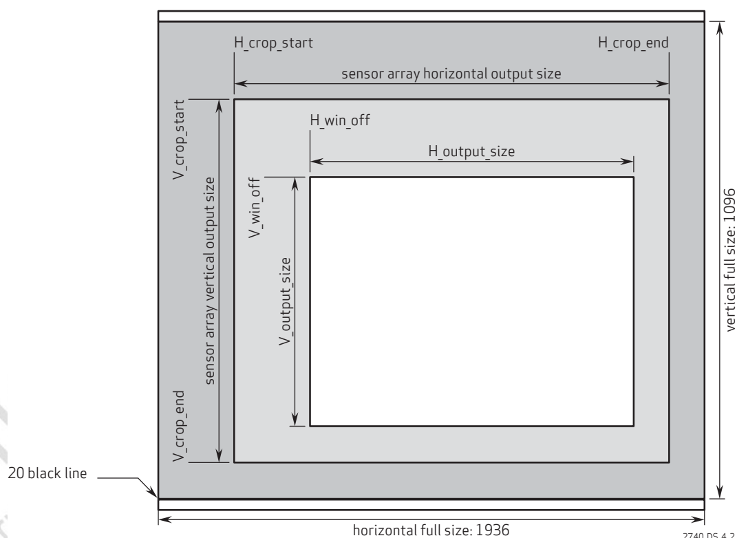
figure 4-2 image windowing
