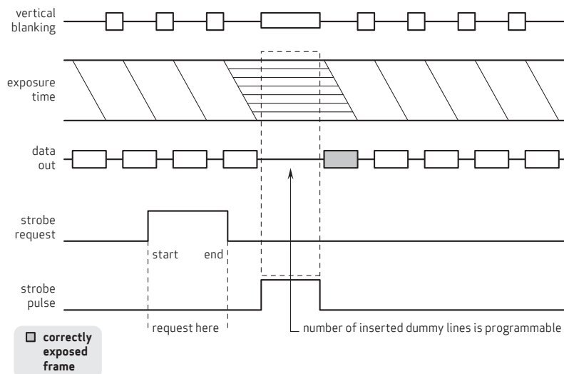
figure 4-9 LED 1 mode
