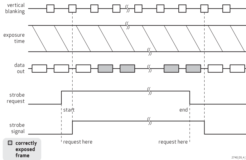
figure 4-11 LED 3 mode
