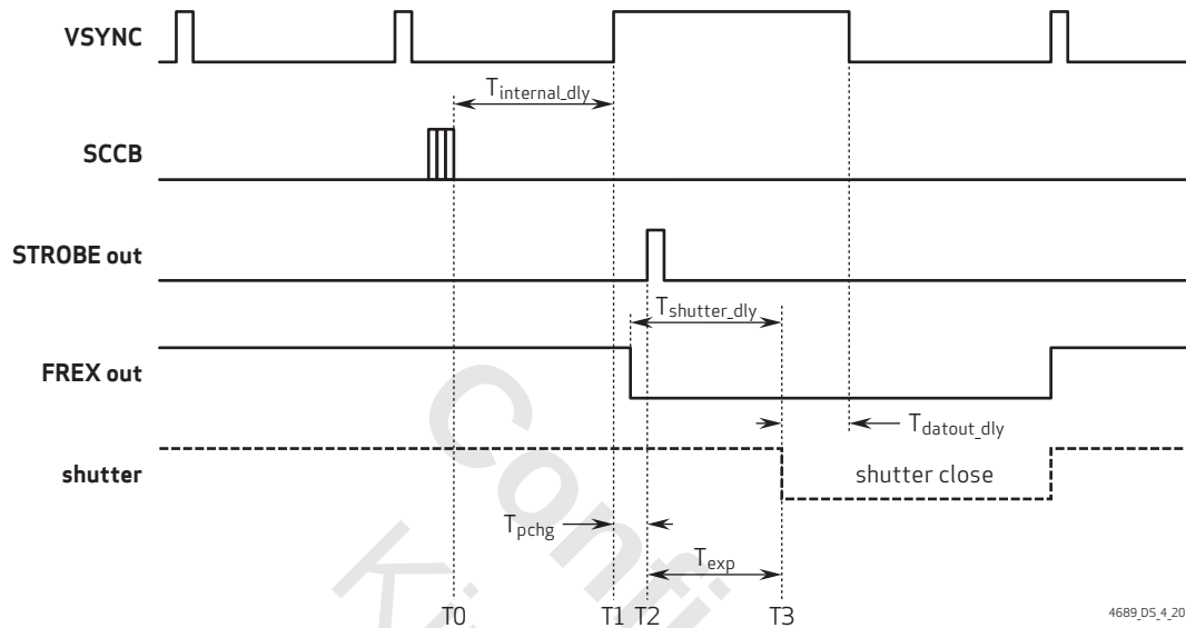
figure 4-17 FREX mode 2 (shutter delay > 0) timing diagram
