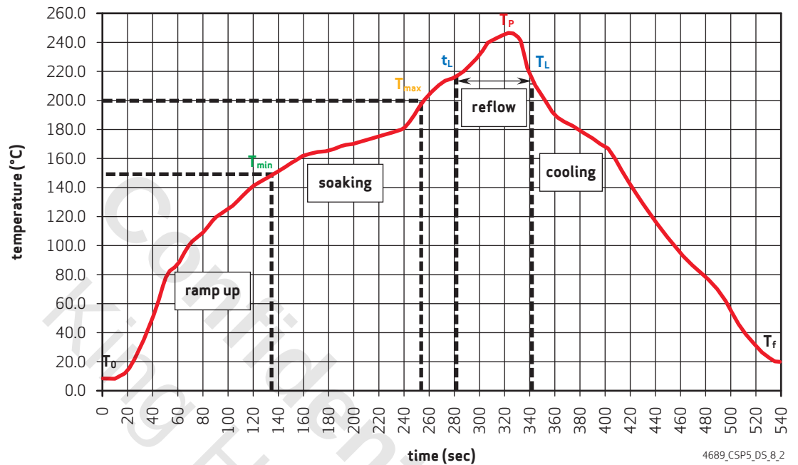
figure 8-2 IR reflow ramp rate requirements
