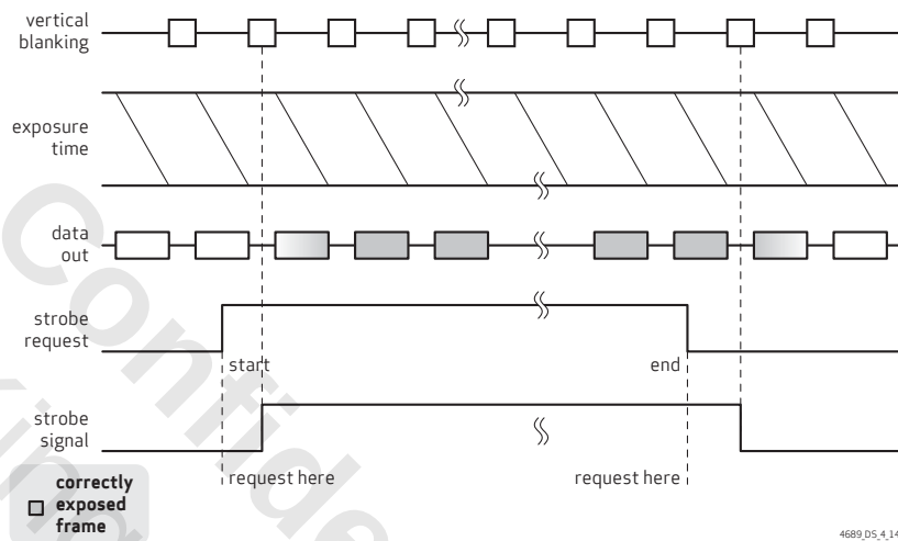
figure 4-11 LED 3 mode
