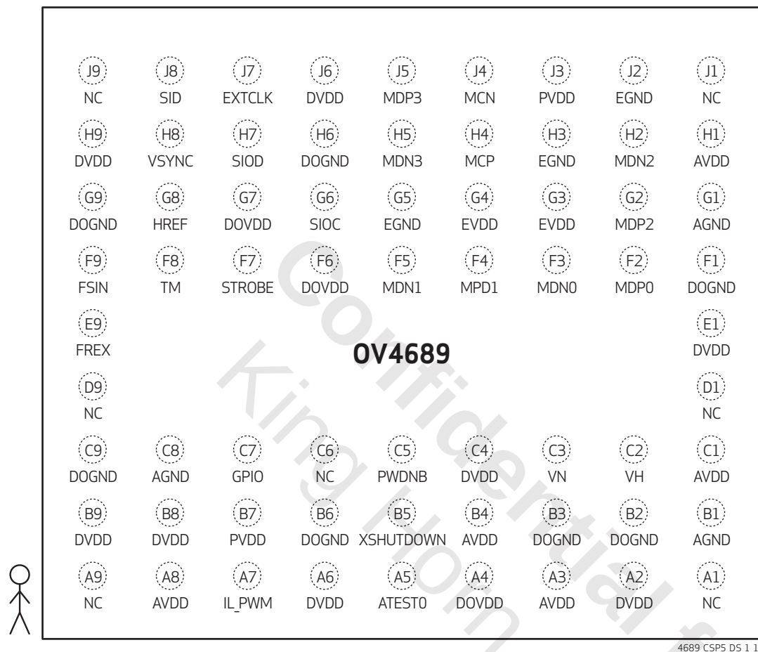
figure 1-1 pin diagram
