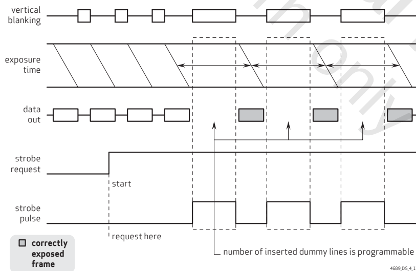
figure 4-10 LED1/LED2 multi-frame mode
