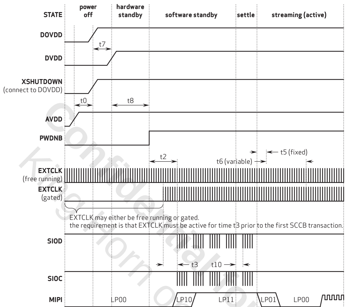
figure 2-4 power up sequence (case 2)
