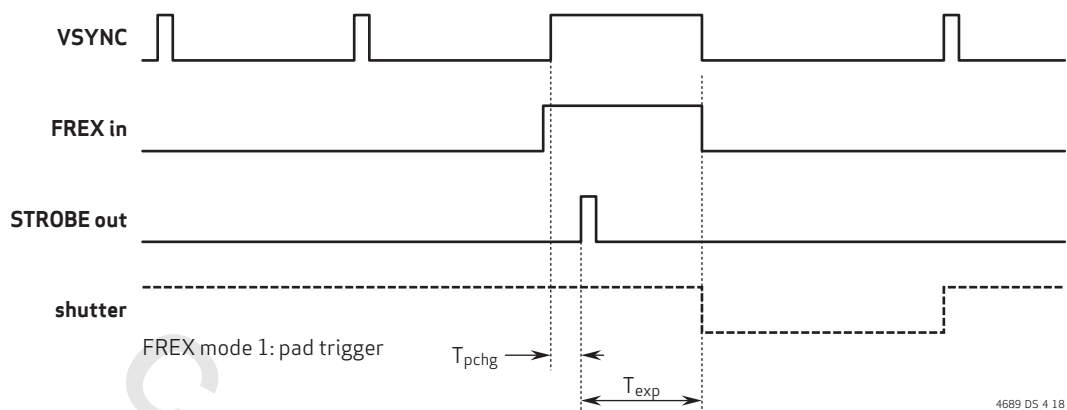
figure 4-15 FREX mode 1 timing diagram
