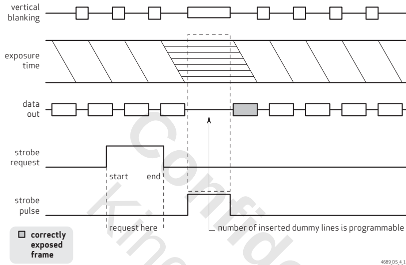
figure 4-9 LED 1/LED 2 single frame mode
