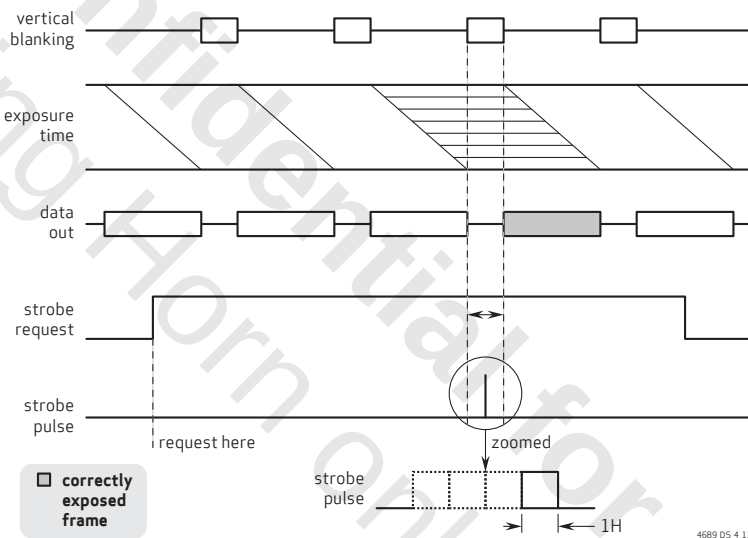
figure 4-8 xenon flash mode
