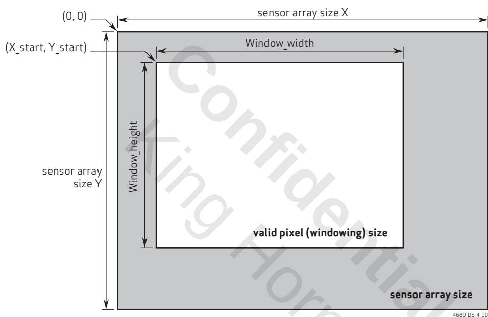
figure 4-7 average-based window definition
