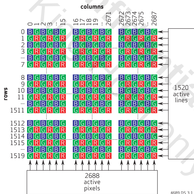
figure 3-1 sensor output pattern (2688x1520)
