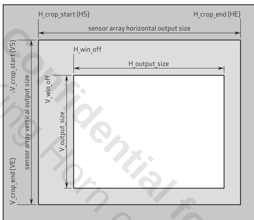
figure 4-2 image cropping and windowing
