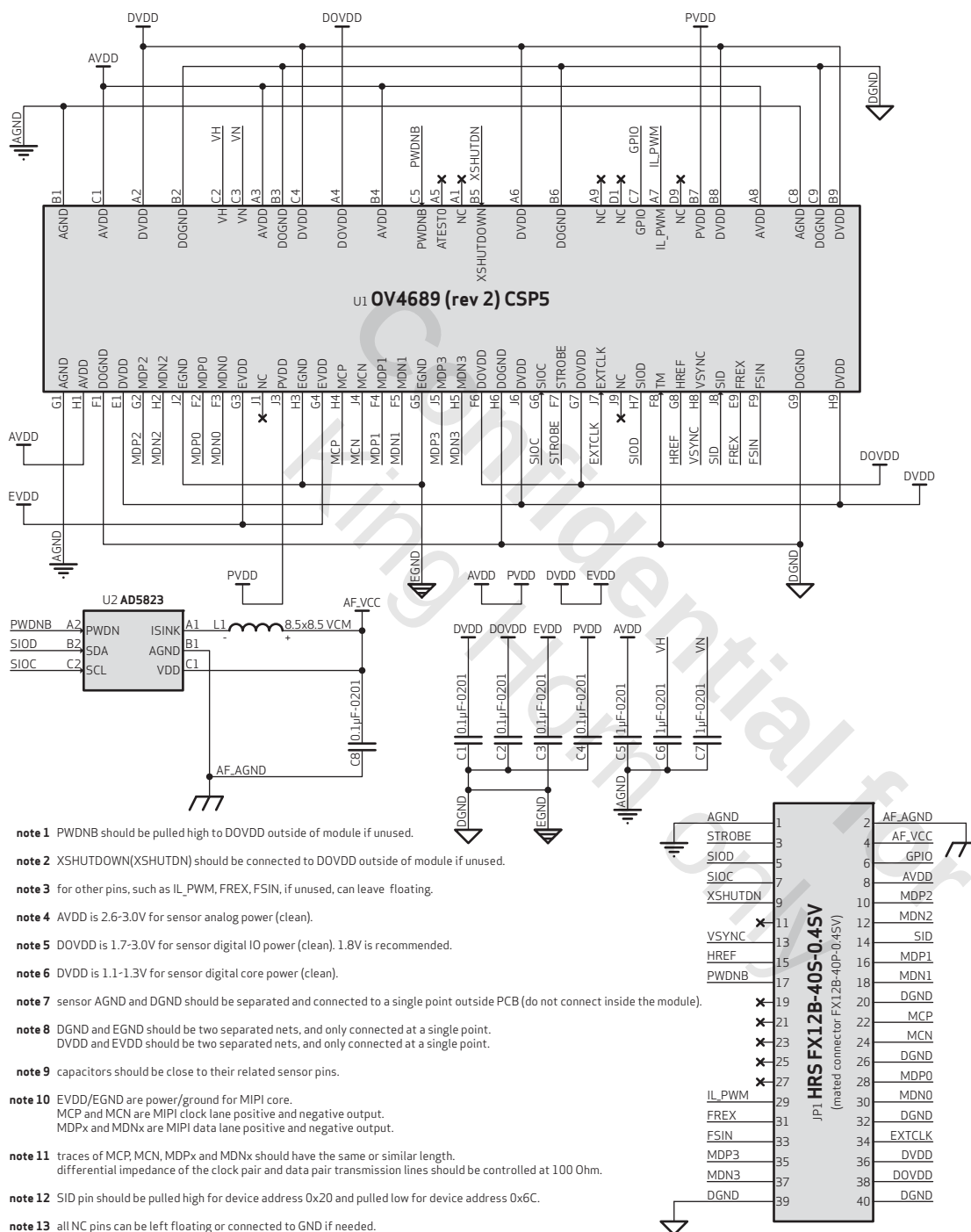
figure 2-2 reference schematic
