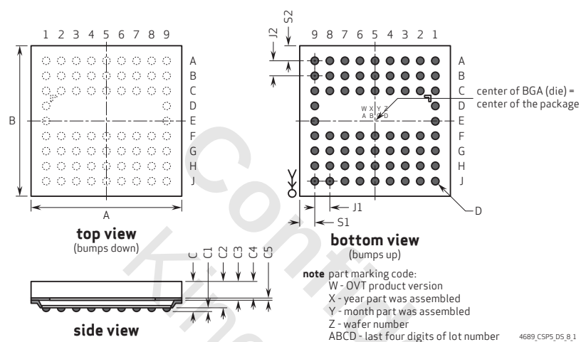
figure 8-1 package specifications
