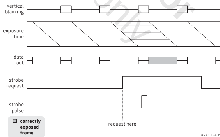
figure 4-12 LED 4 mode
