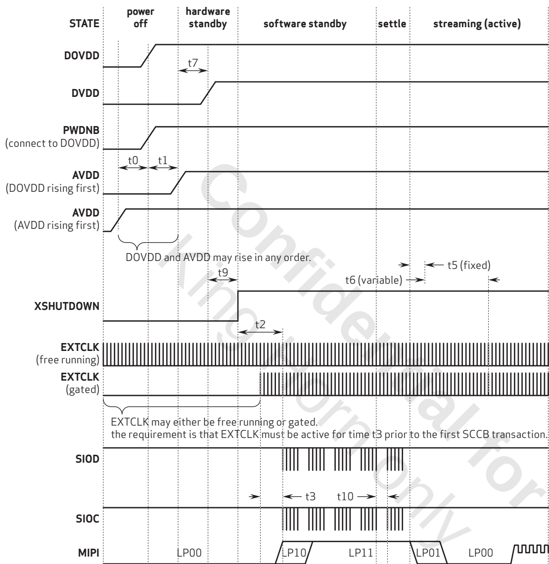
figure 2-3 power up sequence (case 1)
