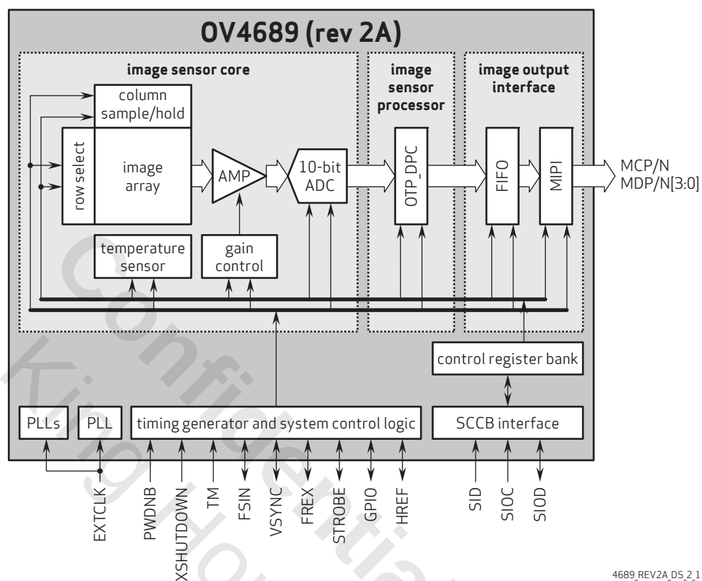
figure 2-1 OV4689 block diagram
