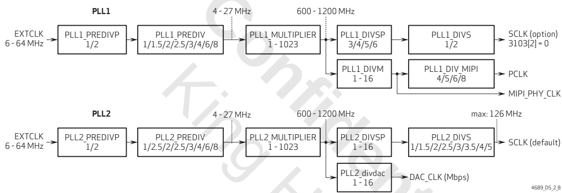
figure 2-8 PLL structure
