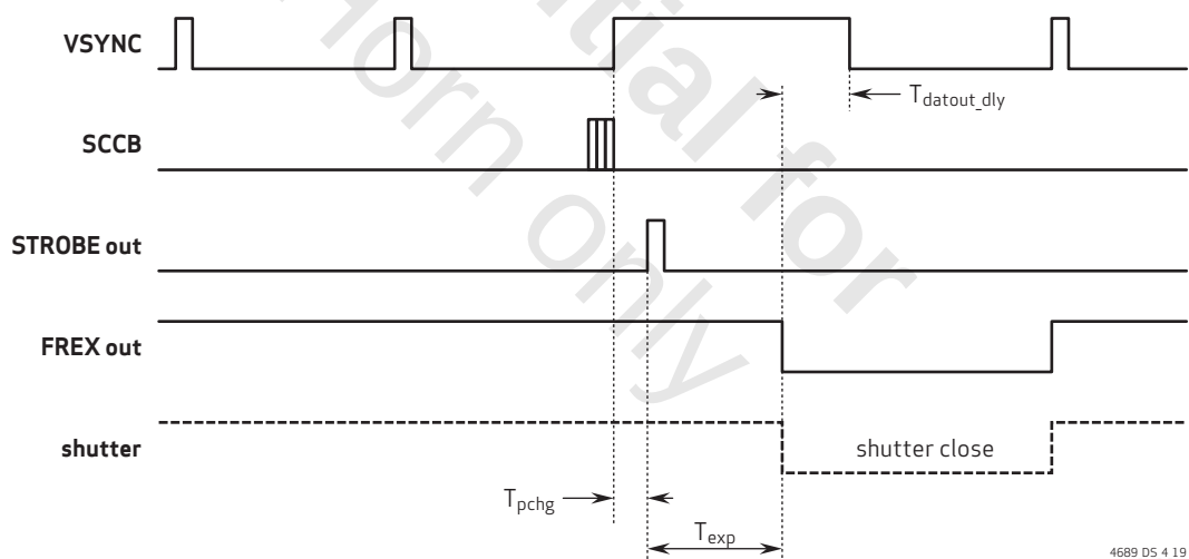
figure 4-16 FREX mode 2 (shutter delay = 0) timing diagram
